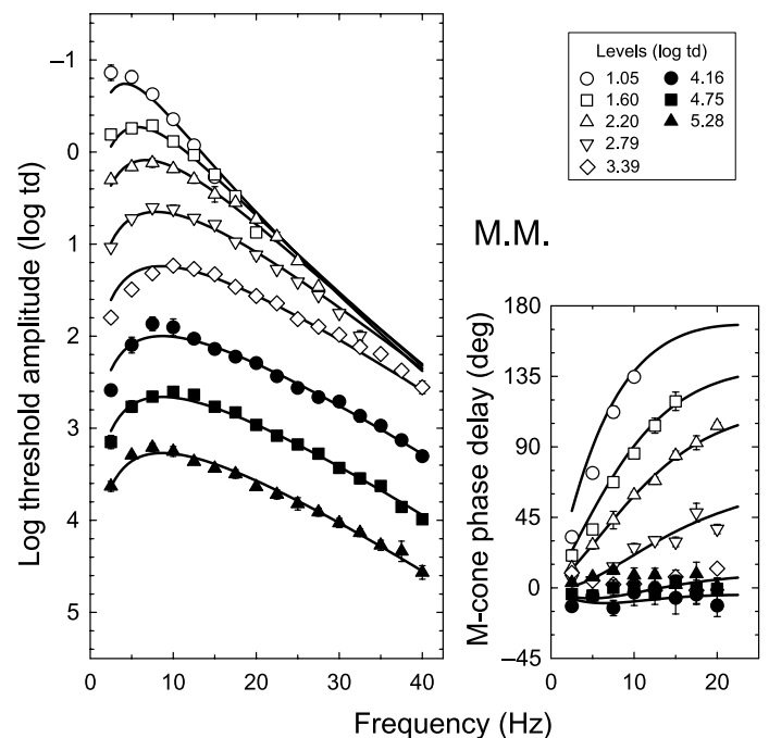
Figure 11. Logarithmic threshold amplitudes and phase delays for M.M. and predictions of Model 2. Details are the same as Figure 10.
