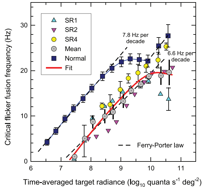
FIGURE 4. S-cone critical flicker fusion frequencies measured on a 620-nm background of 11.41 log 10 quanta s -1 deg -2 are plotted as a function of the mean log radiance of the 440-nm flickering target. Only 3 CRDSR observers participated in this experiment: SR1 ( blue triangles ), SR2 ( purple inverted triangles ), and SR4 ( yellow circles ). The mean CRDSR data ( grey dotted circles ) and the mean data for 12 normal observers ( dark-blue squares ) are also shown. The continuous blue curve through the dark-blue squares provides a template for the normal data. The red line is a shifted scaled version of this template as described in the text. The error bars are ±1 SEM within observers for the individual CRDSR data, and between observers for the mean data. The dashed black lines are best-fitting linear slopes fitted to the mean data for normals and affected observer over the range of radiances over which the Ferry-Porter law holds. The best-fitting slopes are 7.8 Hz per decade for normals and 6.6 Hz per decade for the CRDSR observers.
