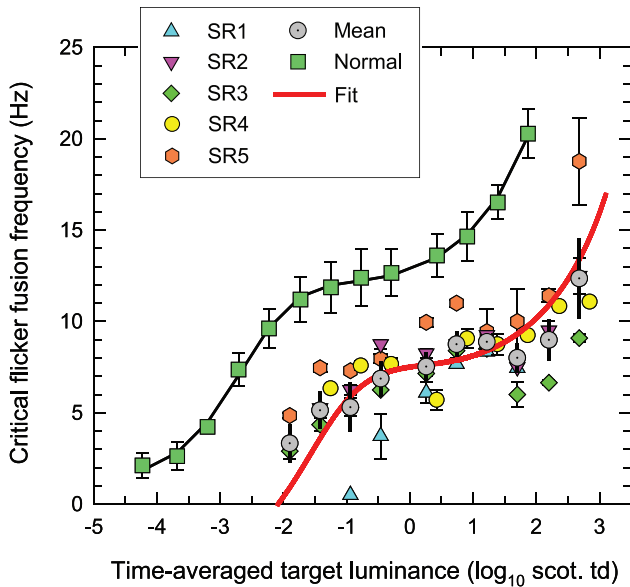
FIGURE 3. Rod critical fusion frequencies ( linear scale ) measured at 10° in the temporal retina are plotted as a function of the mean log 10 scotopic luminance of the 500-nm flickering target. Individual data are plotted for the 5 CRDSR observers: SR1 ( blue triangles ), SR2 ( purple inverted triangles ), SR3 ( green diamonds ), SR4 ( yellow circles ), and SR5 ( orange hexagons ). The mean CRDSR data ( grey dotted circles ) and mean data for 5 normal observers ( green squares ) are also shown. The black curve through the green squares provides a template for the normal data. The red line is a shifted version of this template as described in the text. The error bars are ±1 SEM within observers for the individual CRDSR data, and between observers for the mean data.
