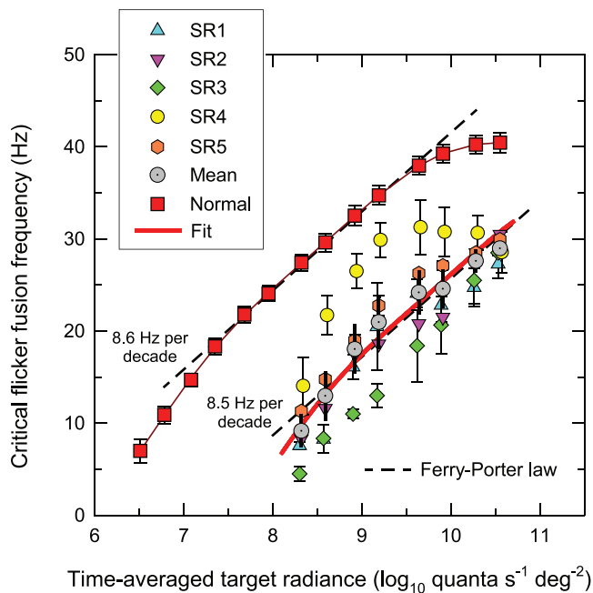
FIGURE 1. L-cone critical flicker fusion frequencies ( linear scale ) measured on a 481-nm background of 8.26 \log_{10} \text{ quanta s}^{-1} \text{ deg}^{-2} are plotted as a function of the mean \log_{10} radiance of a 650-nm flickering target. Data are plotted for 5 CRDSR observers: SR1 ( blue triangles ), SR2 ( purple inverted triangles ), SR3 ( green diamonds ), SR4 ( yellow circles ), and SR5 ( orange hexagons ). The mean CRDSR data ( grey dotted circles ) and mean data for 12 normal observers ( red squares ) are also shown. The thin red line through the red squares provides a template for the normal data. The thicker red line is a shifted version of this template as described in the text. The error bars are \pm 1 SEM within observers for the individual CRDSR data, and between observers for the mean data. The dashed black lines are best-fitting linear slopes fitted to the mean data for normals and affected observer over the range of radiances over which the Ferry-Porter law holds (see text for details). The best-fitting slopes are 8.6 Hz per decade for normals and 8.5 Hz per decade for the CRDSR observers.
