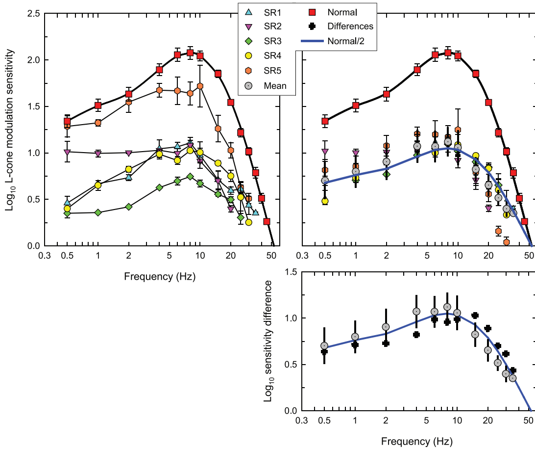
FIGURE 2. Left: Log 10 L-cone modulation sensitivities measured by using a sinusoidally modulated 650-nm target fixed at a radiance of 10.28 log quanta s -1 deg -2 superimposed on a 480-nm background of 8.29 log 10 quanta s -1 deg -2 (1.42 log 10 photopic trolands or 2.58 log 10 scotopic trolands) are plotted as a function of temporal frequency (logarithmic axis). Data are plotted for the 5 CRDSR observers: SR1 (blue triangles), SR2 (purple inverted triangles), SR3 (green diamonds), SR4 (yellow circles), and SR5 (orange hexagons). The mean data for 8 normal observers (red squares) are also shown. Upper right: The log 10 L-cone modulation sensitivities for the individual CRDSR observers vertically aligned by using a least-squares fitting procedure with the mean CRDSR data (grey dotted circles). The logarithmic mean normal data are replotted as in the left (red squares) but also divided by two (blue line). Lower right: The logarithmic mean normal data divided by two (blue line) compared with the differences between the mean normal and CRDSR data (black crosses). The error bars are ±1 SEM within observers for the individual CRDSR data, and between observers for the mean data.
